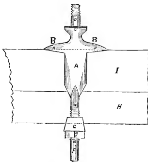
PHELPS'S KING-BOLT.
